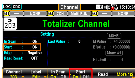
Start - On
