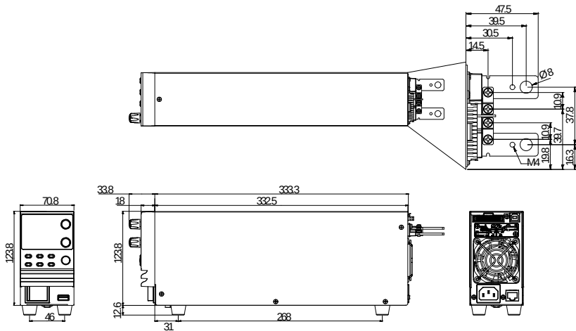
Type I PSW-360M160/PSW-360L80/PSW-360L30 (mm)
